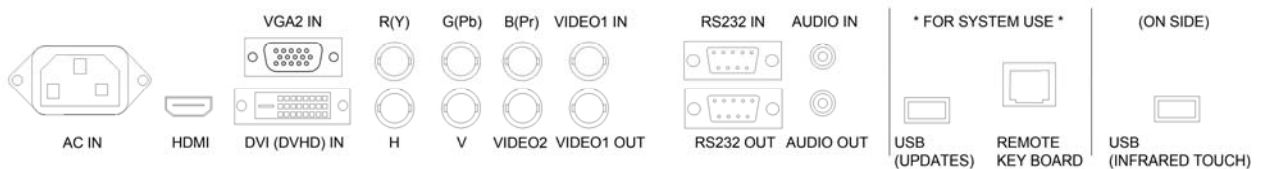
Figure 4 Screen Inputs
